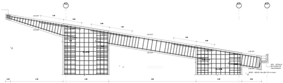
VIGA V-8B (0.25X0.60) -AZOTEA
